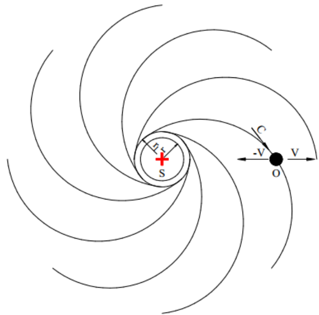
Figure. 1. S - light source (the atom), O - observer, r - radius of the atom, r_l - the radius of the orbit of the highest flux at his address in a calm state, prior to heating (at orbital velocity), v - relative velocity of removal or approximation between S and O, c - velocity of light vector.
