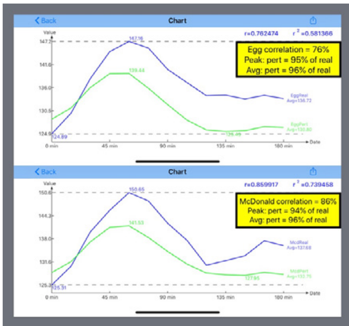
Figure 3: Comparison between perturbed and measured PPG for both egg and McDonalds' breakfasts
