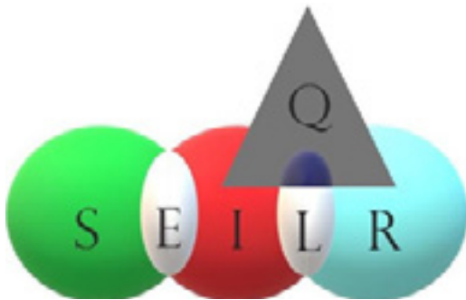
Figure 4: Resume of Fig.1,2,3
