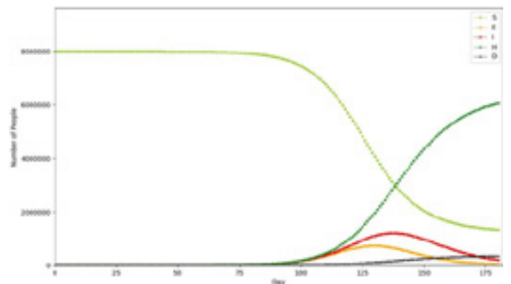
Figure 12: Result of SEIR simulation
