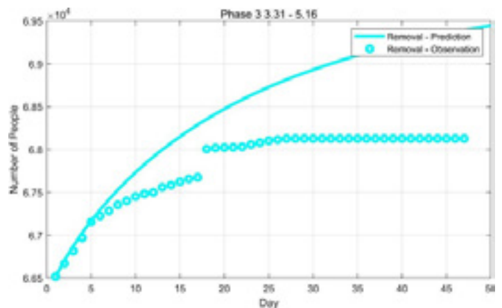
Figure 11: Result of curve fitting for the removal R(t) in Phase 3 (2020.3.31-2020.5.16)
