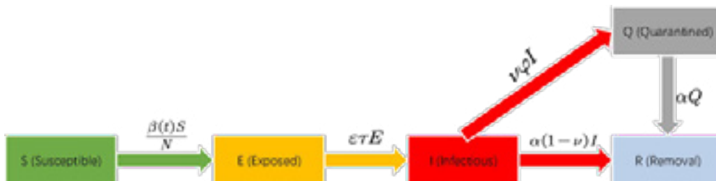
Figure 2: 2020.2.8 - 2020.3.30, SEIQR model, where \beta(t) = \beta(wE+I+Q)
