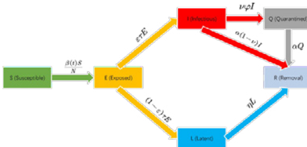
Figure 3: 2020.3.31 - 2020.5.16, SEIQLR model, where \beta(t) = \beta(wE+I+Q+\lambda L)
